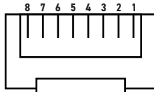
RJ45 8-pol.
